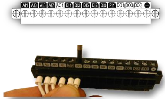
Figure 4. Positive identification on removable terminals
